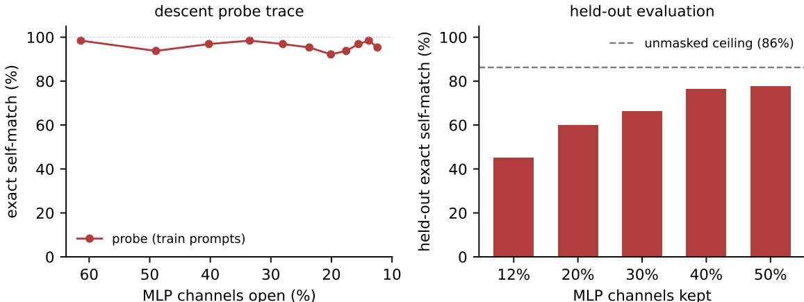
Figure 3: Function calling, Qwen3-4B. Left: probe trace during descent — exact self-match holds at 92–98% from 61% open down to 12% open on training prompts. Right: held-out self-match by budget; the dashed line is the unmasked adapted model’s own self-match (86%), which upper-bounds every masked number.
