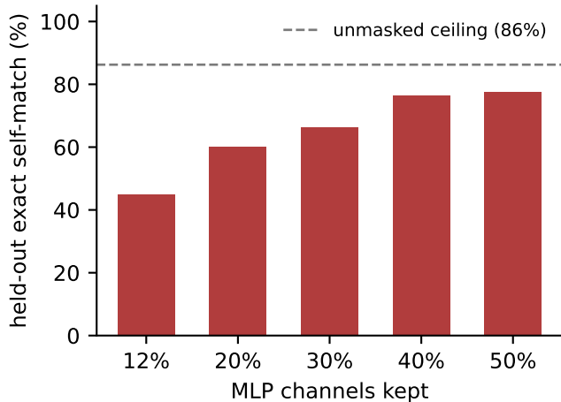
held-out evaluation
