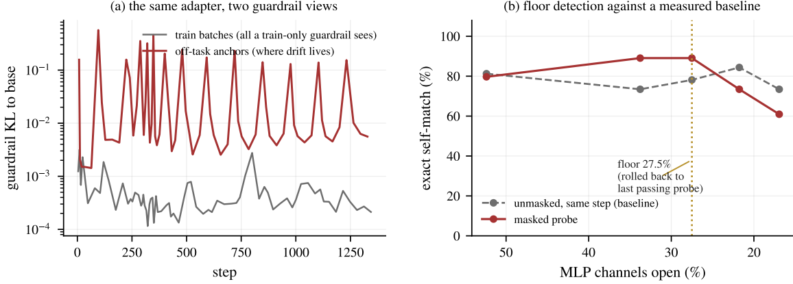
Figure 7: Two failure modes, instrumented (JSON extraction run). (a) Guardrail KL on train batches (gray) vs. rotating off-task anchor batches (red), same adapter and same steps: the train-batch view reads 10–100× lower than the anchor view. Drift lives exactly where a train-only guardrail cannot see it. (b) Floor detection: the masked probe (red) is compared against the unmasked model measured at the same step (gray, itself depressed by decode noise and residual drift), never against an assumed 100%. When the masked probe falls below tolerance twice, the gates roll back to the last passing sparsity.
