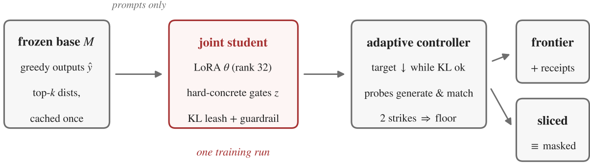
Figure 1: One-shot extraction. The frozen base model supplies label-free targets (greedy outputs and cached top- k distributions); gates and adapter train jointly under a KL leash; an adaptive controller paced by generation probes finds the floor; the run emits the sparsity–fidelity frontier, integrity receipts, and a physically sliced model.
