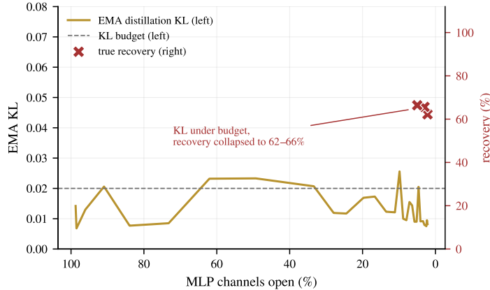
Figure 5: The failed KL-only controller (v2.0): EMA distillation KL stays under budget throughout the descent (left axis) while true held-out recovery collapses (crosses, right axis). Generation probes detect this; losses do not.
