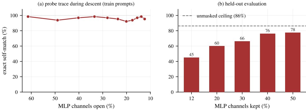
Figure 4: Function calling, Qwen3-4B. Left: probe trace during descent — exact self-match holds at 92–98% from 61% open down to 12% open on training prompts. Right: held-out self-match by budget; the dashed line is the unmasked adapted model’s own self-match (86%), which upper-bounds every masked number.
