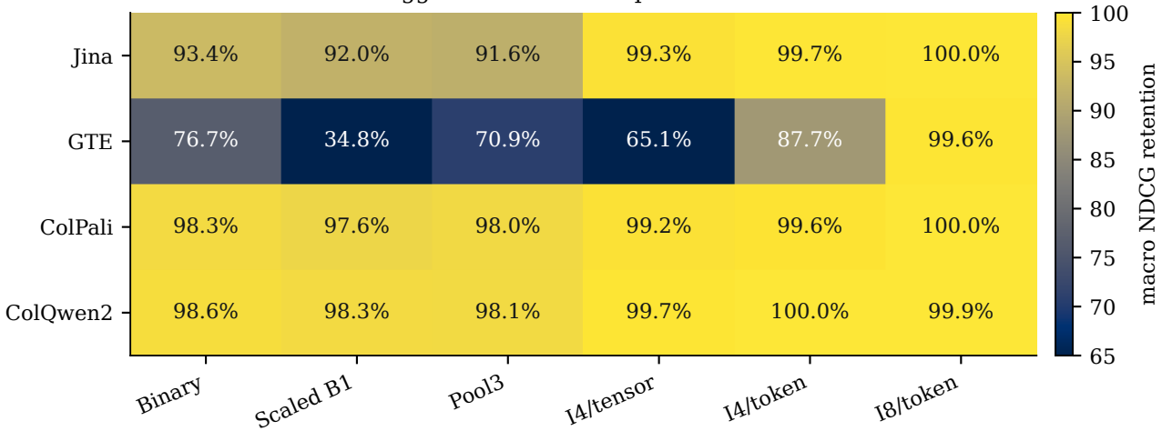
The best aggressive format depends on the encoder
