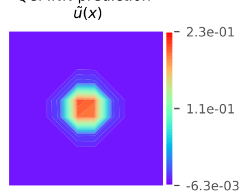
QCPINN prediction
