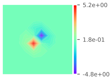
\hat{f}(x)
