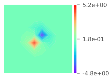
\tilde{f}(x)
