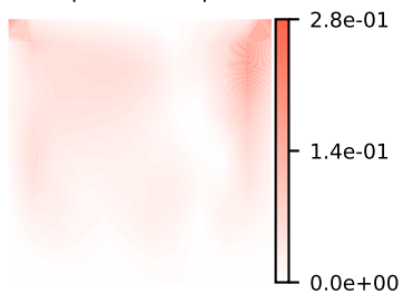
|v(x) - \hat{v}(x)|
