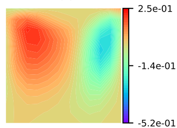
\tilde{v}(x)
