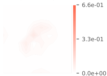
|f(x) - \tilde{f}(x)|
