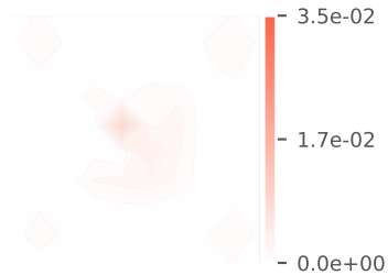
|u(x) - \tilde{u}(x)|
