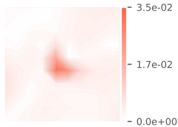
|u(x) - \hat{u}(x)|
