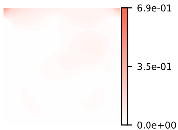
|u(x) - \hat{u}(x)|
