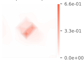
|f(x) - \hat{f}(x)|
