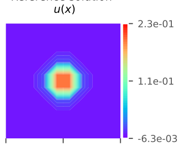
Reference solution
