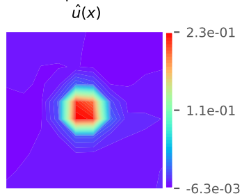
PINN prediction
