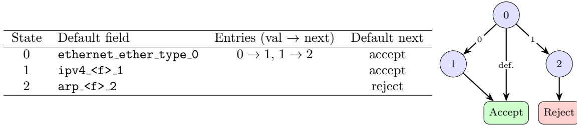
Figure 3.5: The synthesised FSM for the running example's .pc program for the first design. Left: the state-table representation. Right: the corresponding state-transition graph. State numbers in the graph match the rows of the table.
