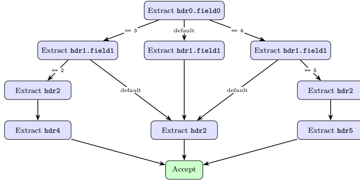
Figure 3.7: The FSM after stitching back hdr2 , hdr4 and hdr5 . The state extracting hdr2 on the default paths is shared.
