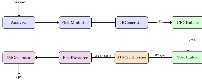
Figure 3.2: The synthesis pipeline. Boxes are colour-coded by phase: frontend (blue), specification construction (green), synthesis (orange), and backend (violet).
