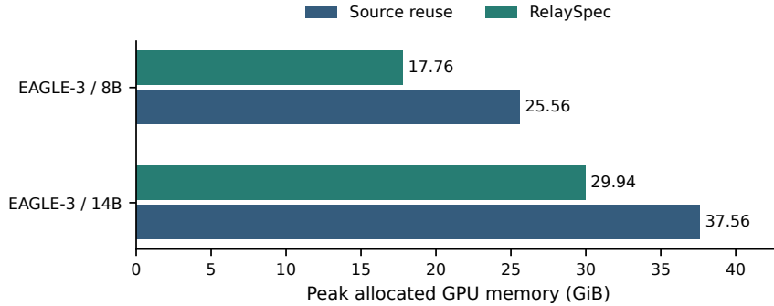
Figure 12: Isolated EAGLE-3 peak allocated memory on RTX 6000 Ada. Each method runs in a fresh process on eight paired prompts per target. Source removal saves 7.80 GiB at 8B and 7.63 GiB at 14B.
