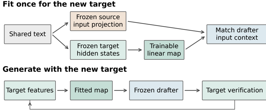
Figure 1: Fit once, then reuse the frozen drafter. The source and target process identical text during fitting. Only the map is updated. During generation, target features from committed positions feed the next draft.
