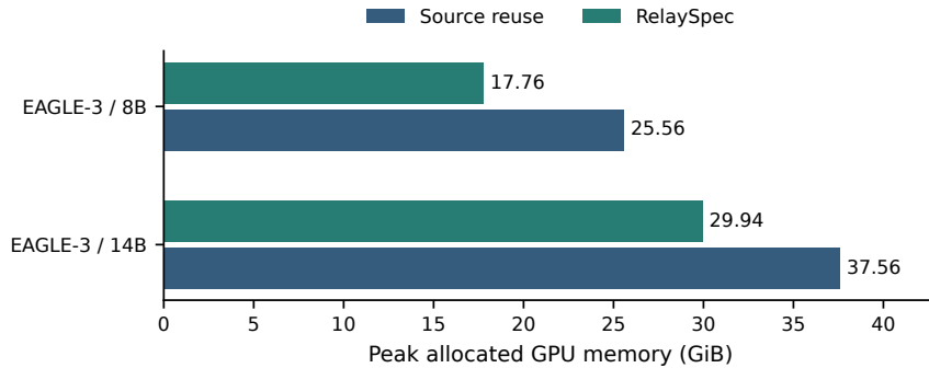
Figure 16: Isolated EAGLE-3 peak allocated memory on RTX 6000 Ada. Each method runs in a fresh process on eight paired prompts per target. Source removal saves 7.80 GiB at 8B and 7.63 GiB at 14B.
