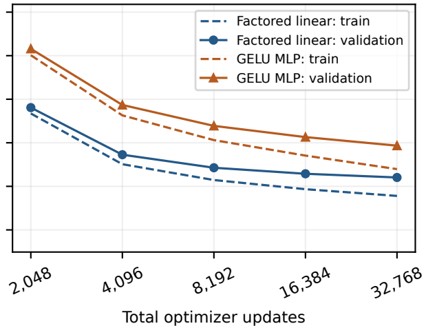
Width 512; 2,048 fitting records
