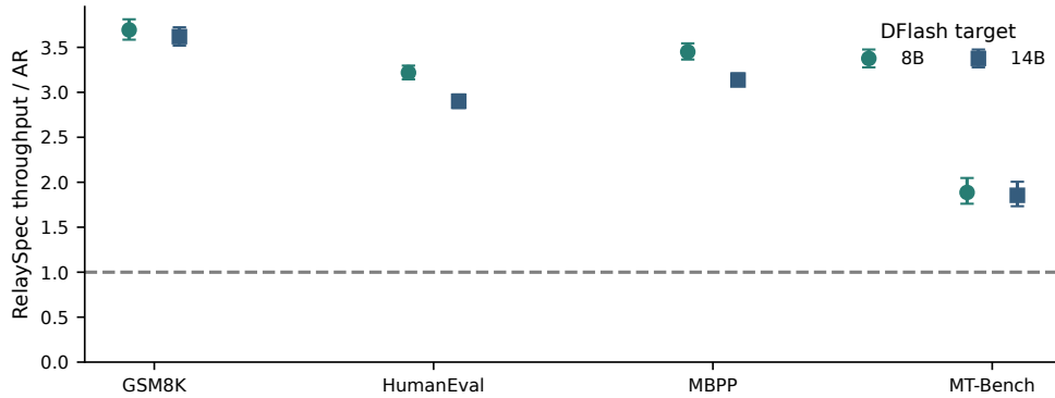
Figure 5: DFlash RelaySpec throughput relative to AR across workloads. Whiskers are paired 95% intervals. Chat intervals resample whole two-turn conversations. Full absolute values are in Table 9.
