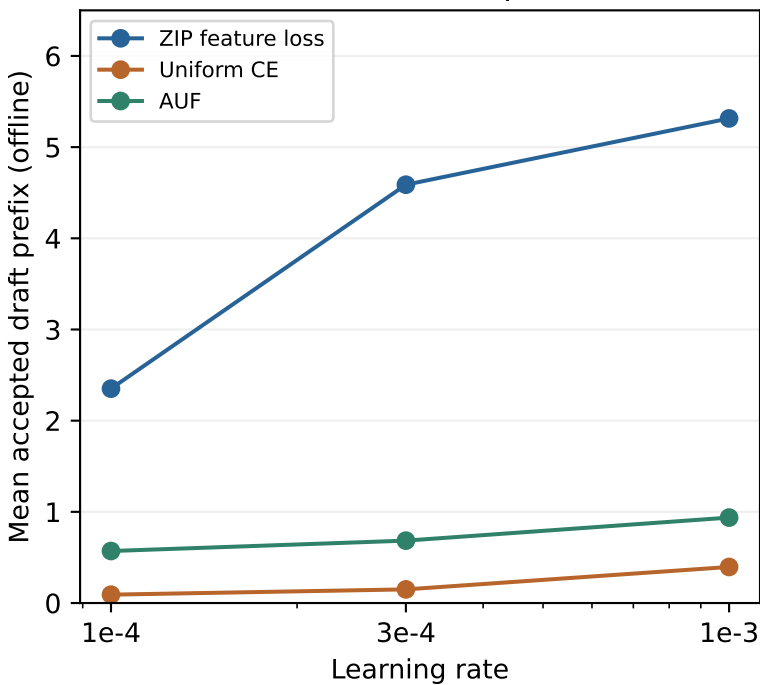
512 records, 3 epochs
