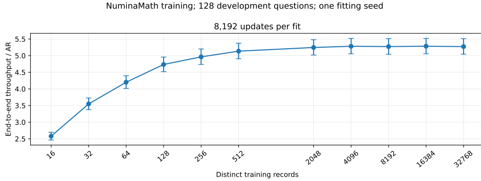
Figure 2: DFlash-8B data scaling on 128 development questions, with NuminaMath training and 8,192 updates per fit. All dataset sizes are measured with shared controls in one campaign. Paired 95% request intervals exclude fitting-seed variation and selection uncertainty.
