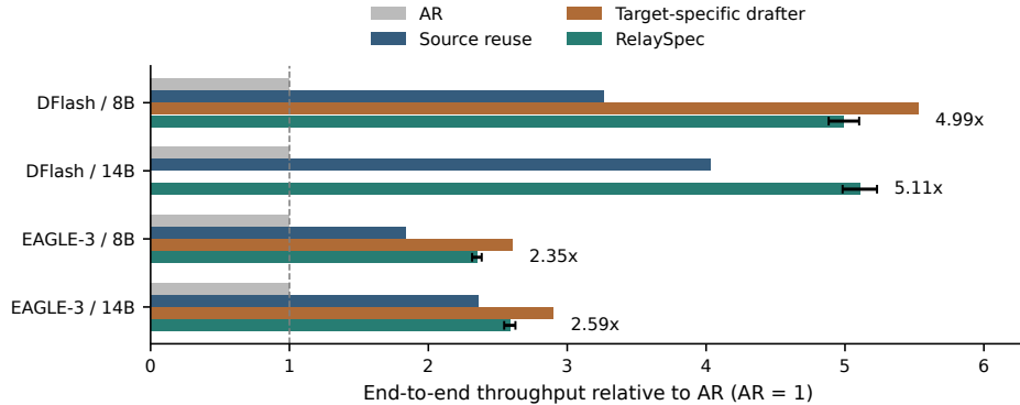
Figure 4: MATH-500 throughput relative to plain AR, measured within each paired run. RelaySpec reuses the 4B drafter. The native control uses a drafter released for the evaluated target. Whiskers show RelaySpec’s 95% paired intervals. Native controls show the three evaluated releases. Each runtime uses one request per GPU.
