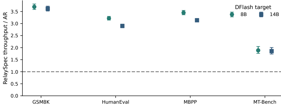
Figure 5: DFlash RelaySpec throughput relative to AR across workloads. Whiskers are paired 95% intervals. Chat intervals resample whole two-turn conversations. Full absolute values are in Table 11.
