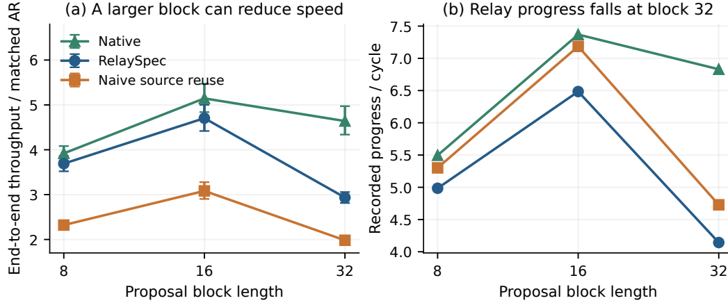
Figure 9: DFlash-8B block-size screen on 64 development questions, 512-output-token cap, RTX 6000 Ada. Larger blocks do not guarantee more accepted progress or higher speed. (a) End-to-end throughput relative to each block run’s AR with paired 95% request intervals. (b) Recorded target-token progress per cycle. The source baseline here is naive source reuse.
