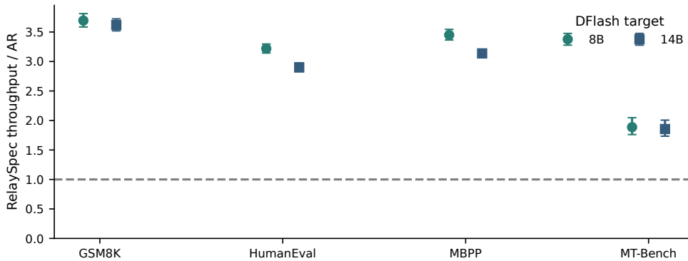
Figure 8: DFlash RelaySpec throughput relative to AR across workloads. Whiskers are paired 95% intervals. Chat intervals resample whole two-turn conversations. Full absolute values are in Table 9.
