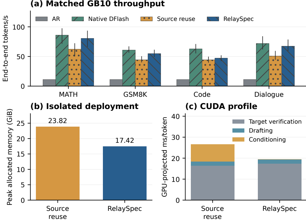
Figure 29: RelaySpec on GB10. (a) Throughput by workload with paired-request 95% intervals, eight requests per workload. (b) Peak PyTorch allocated memory in isolated deployments. (c) Nsight Systems GPU-projected stage time on one warmed MATH request with a 256-token cap. Conditioning is the source transformer or relay mapping. These projected spans are neither unprofiled wall times nor a union of kernel-busy intervals.
