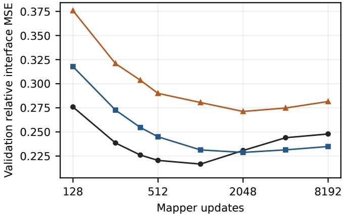
EAGLE-3, N=512
