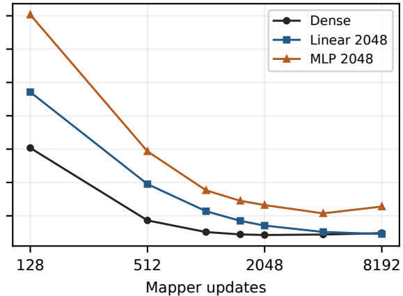
EAGLE-3, N=2,048
