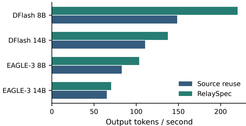
(a) Measured throughput
