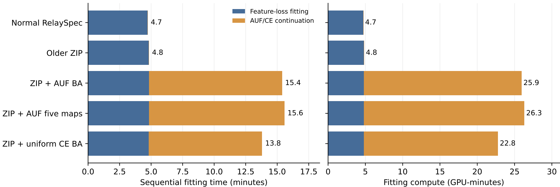
Qwen8 adaptation: measured fitting cost on 4,096 records
