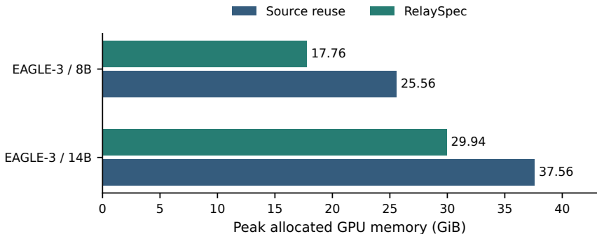
Figure 14: Isolated EAGLE-3 peak allocated memory on RTX 6000 Ada. Each method runs in a fresh process on eight paired prompts per target. Source removal saves 7.80 GiB at 8B and 7.63 GiB at 14B.
