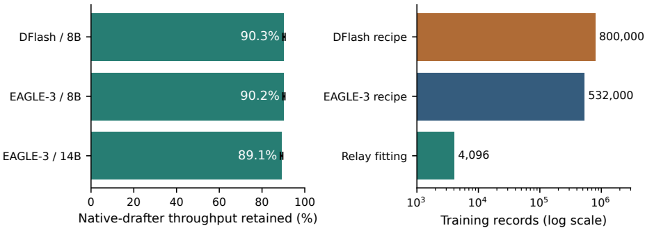
Figure 15: Left: fraction of native target-specific drafter throughput retained by RelaySpec in paired MATH-500 runs. Right: published original DFlash and EAGLE-3 recipe sizes versus the additional RelaySpec fitting set. Recipe counts provide training-scale context, not a matched training experiment or an audit of each released checkpoint.
