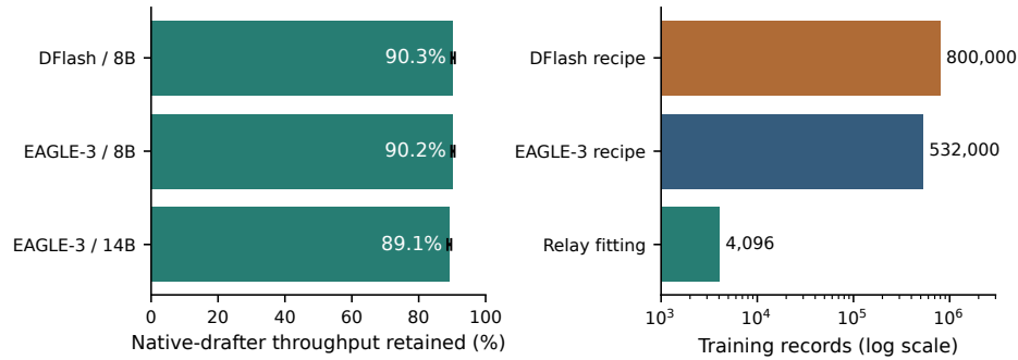
Figure 16: Left: fraction of native target-specific drafter throughput retained by RelaySpec in paired MATH-500 runs. Right: published original DFlash and EAGLE-3 recipe sizes versus the additional RelaySpec fitting set. Recipe counts provide training-scale context, not a matched training experiment or an audit of each released checkpoint.
