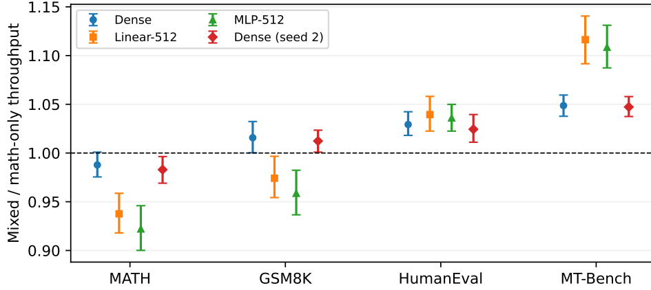
Figure 14: Effect of training composition on measured DFlash-8B throughput. Values above one favor mixed training. Marker shapes distinguish the four matched comparisons. Bars show paired 95% intervals. Code and conversation throughput does not establish output quality.
