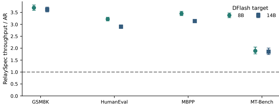
Figure 3: DFlash RelaySpec throughput relative to AR across workloads. Whiskers are paired 95% intervals. Chat intervals resample whole two-turn conversations. Full absolute values are in Table 8.
