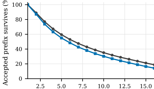
DFlash, target 8B
