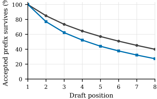
EAGLE-3, target 8B
