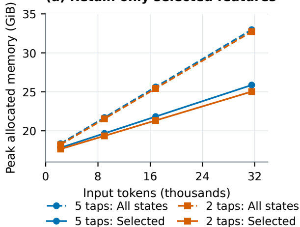
(a) Retain only selected features
