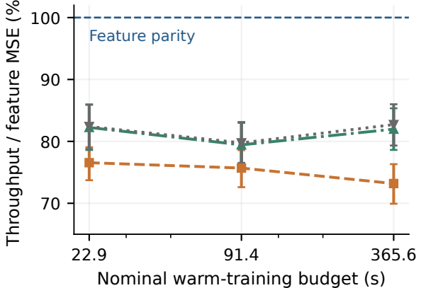
(b) Paired intervals remain below parity
