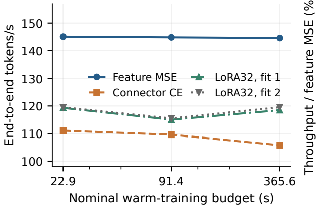
(a) Feature fitting leads at every budget
