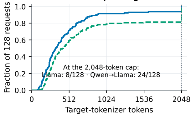
(a) Observed output length
