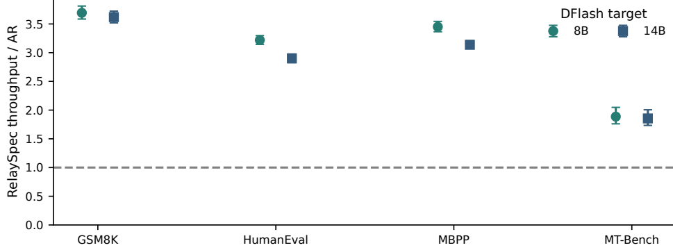
Figure 3: DFlash RelaySpec throughput relative to AR across workloads. Whiskers are paired 95% intervals. Chat intervals resample whole two-turn conversations. Full absolute values are in Table 7.
