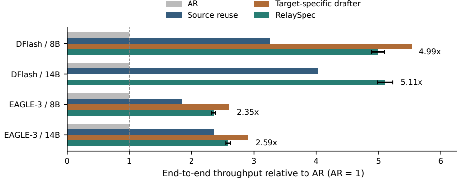
Figure 1: MATH-500 throughput relative to plain AR, measured within each paired run. RelaySpec reuses the 4B drafter. The native control uses a drafter released for the evaluated target. Whiskers show RelaySpec’s 95% paired intervals. Native controls show the three evaluated releases. Each runtime uses one request per GPU.
