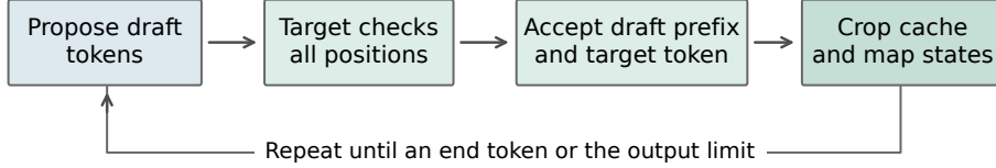
Figure 6: One generation cycle. RelaySpec changes the drafter’s context. The target retains control over committed tokens and the shared decoder retains responsibility for positions, stopping and cache updates.
