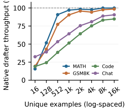
(c) Transfer: 16 to 16k examples
