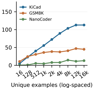
(a) Fine-tuned: 16 to 16k examples
