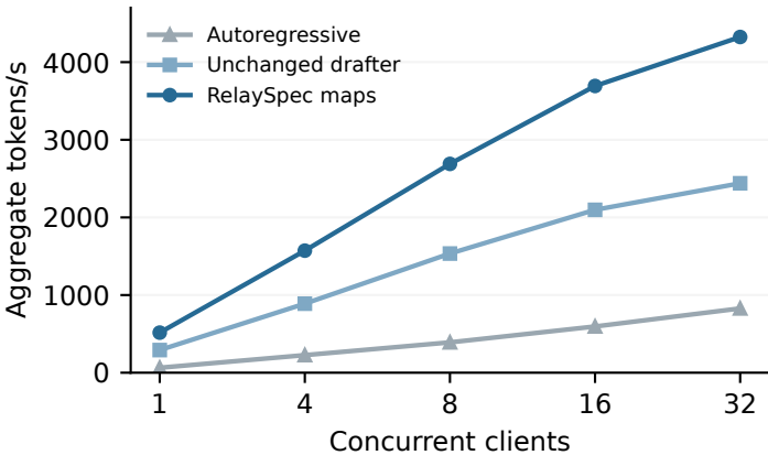
(a) Server throughput
