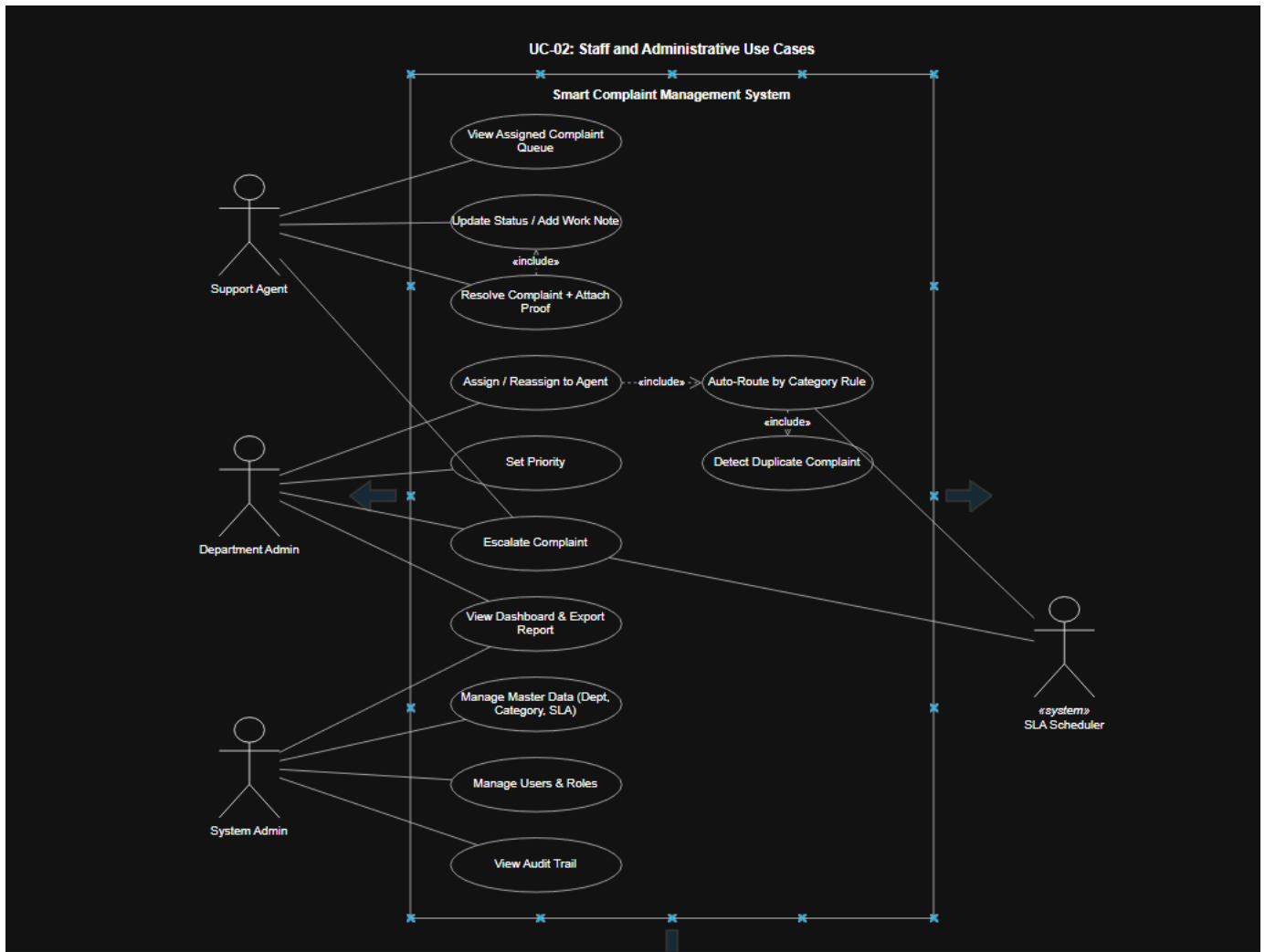
Figure 2: UC-02 — Support Agent, Department Admin, System Admin and the SLA Scheduler. Assignment includes auto-routing, which in turn includes duplicate detection; resolution includes a status update.
