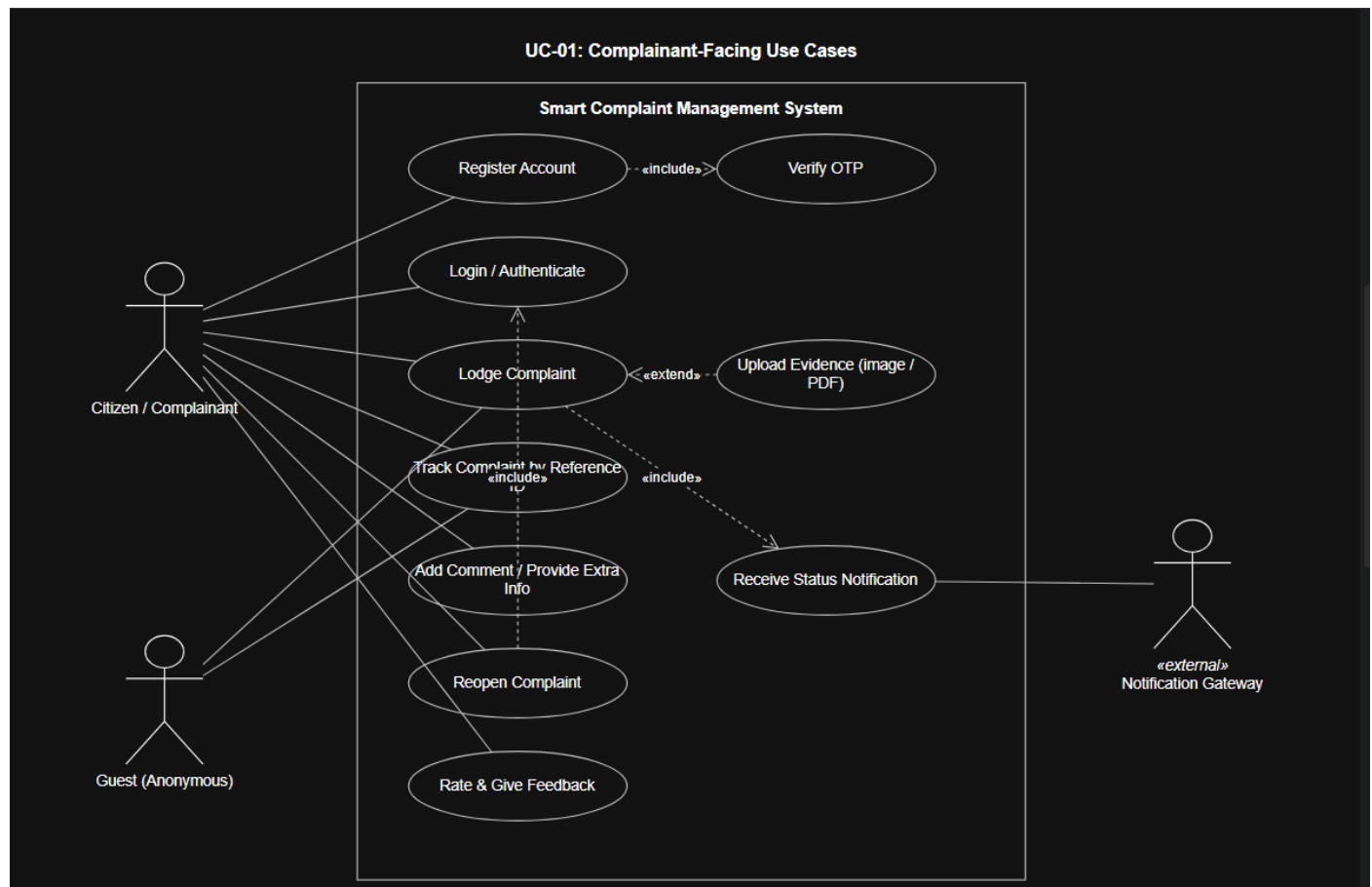
Figure 1: UC-01 — Complainant and guest interaction with SCMS. Registration includes OTP verification; lodging a complaint includes notification and may be extended by evidence upload.
