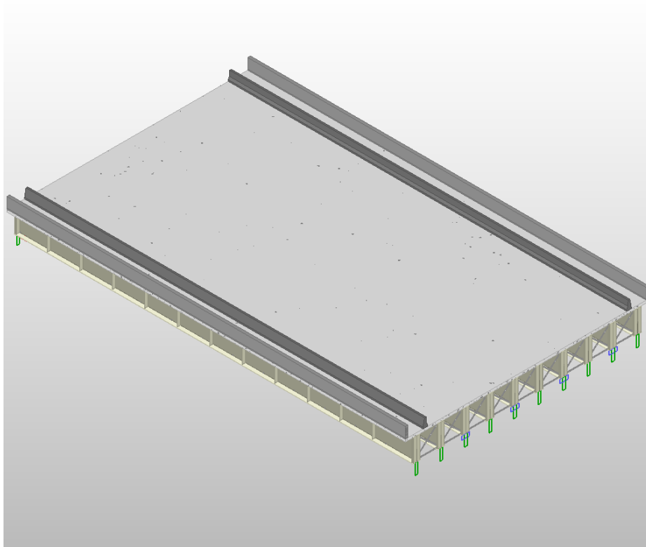
Figure 6.1: Overall 3D Bridge Superstructure
