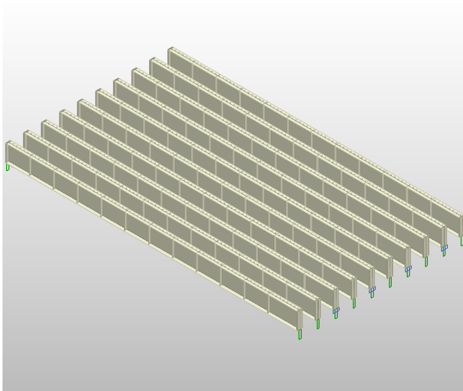
Figure 6.4: 3D View of Plate Girders
