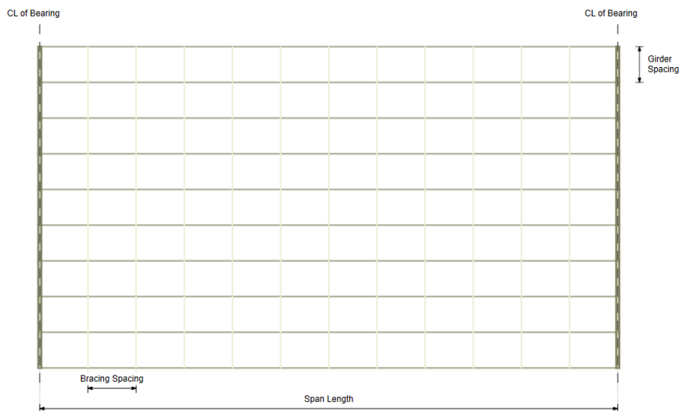
Figure 6.3: Top View
