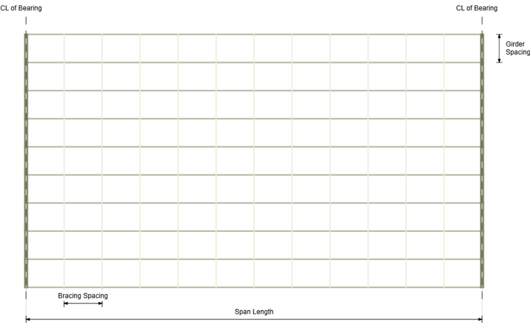
Figure 1 – Overall Bridge Plan
