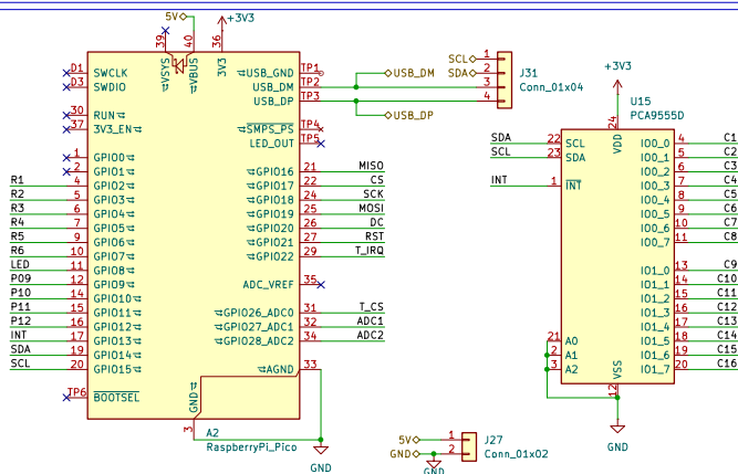
MCU & GPIO EXPANDER
