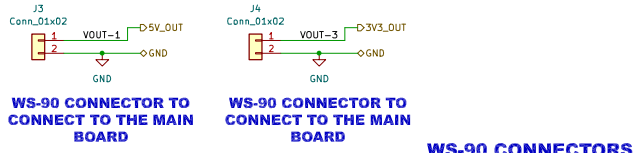
WS-90 CONNECTORS
