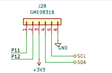
TOUCH PANEL FOR TRACKPAD
