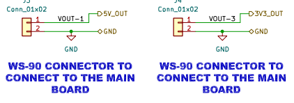
WS-90 CONNECTORS
