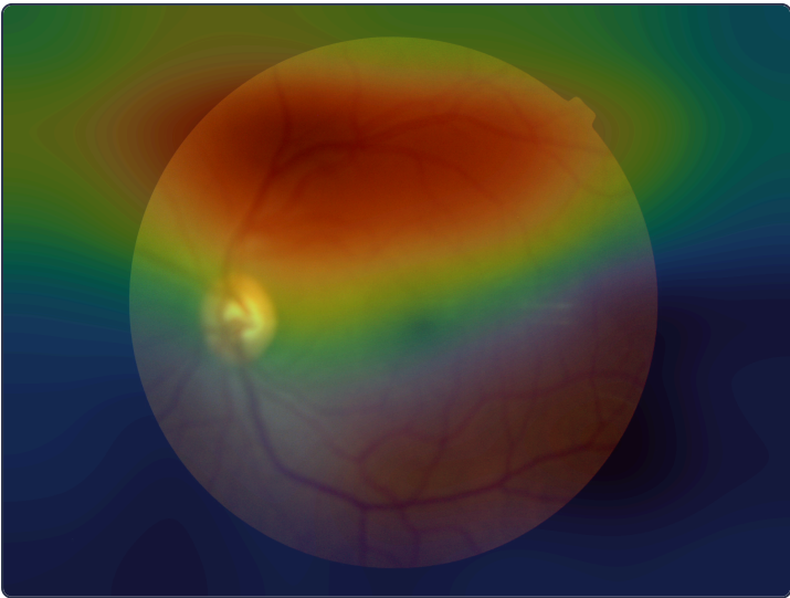
Grad-CAM overlay
