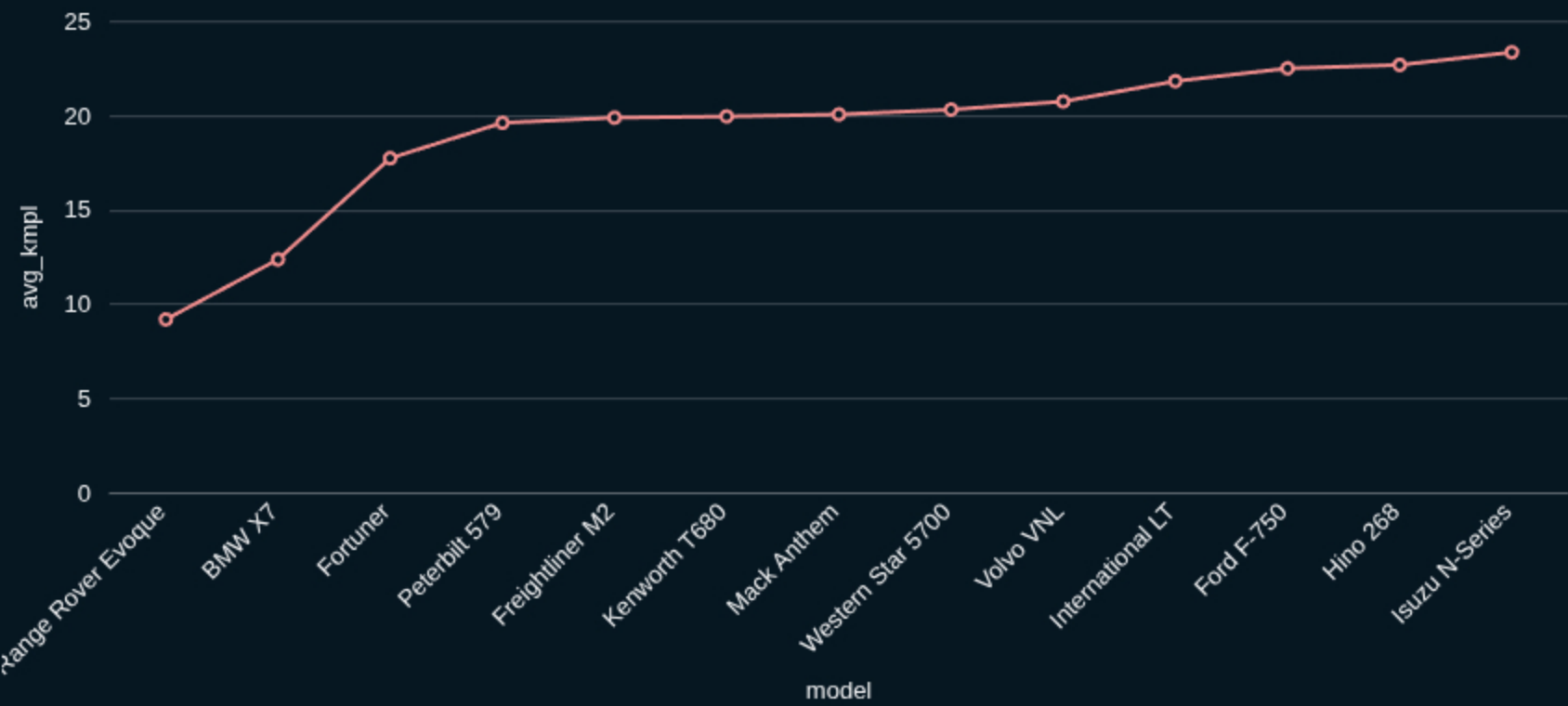
Model-wise Efficiency
