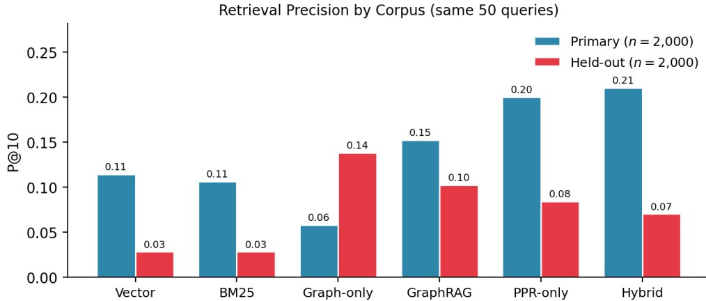
Figure 1: P@10 by system on the primary and held-out corpora. Same 50 queries; system rank order is not significantly correlated across corpora (Kendall \tau = -0.138 , p = 0.702 ).
