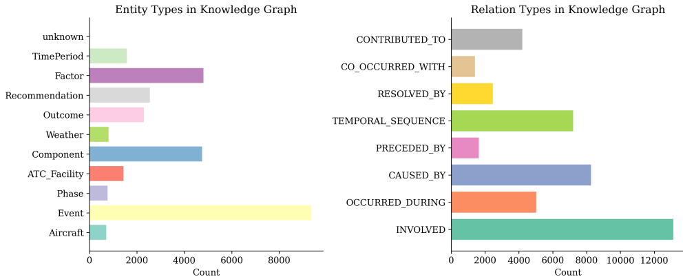
Figure 5: Entity-type and relation-type distributions in the canonicalized knowledge graph.
