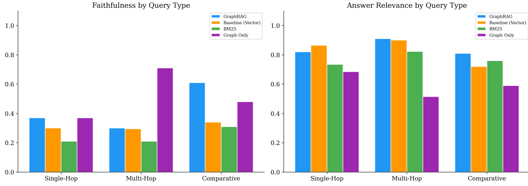
Figure 4: Ollama-judged faithfulness (left) and answer relevance (right) by query type.
