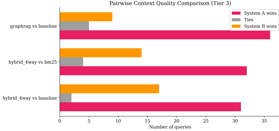
Figure 3: Blind pairwise win rates under the Claude judge for the three comparisons reported in Table 3.
