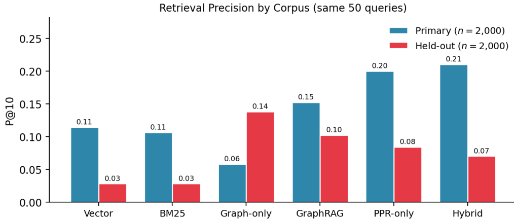
Figure 1: P@10 by system on the primary and held-out corpora. Same 50 queries; system rank order does not correlate across corpora (Kendall \tau = -0.07 ).
