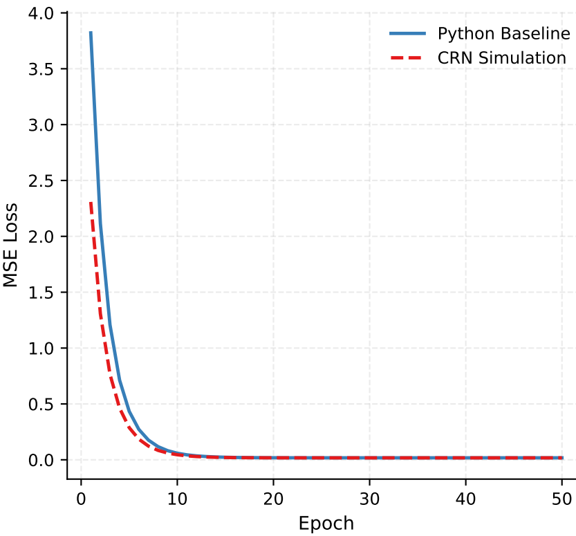
Mean Squared Error Convergence
