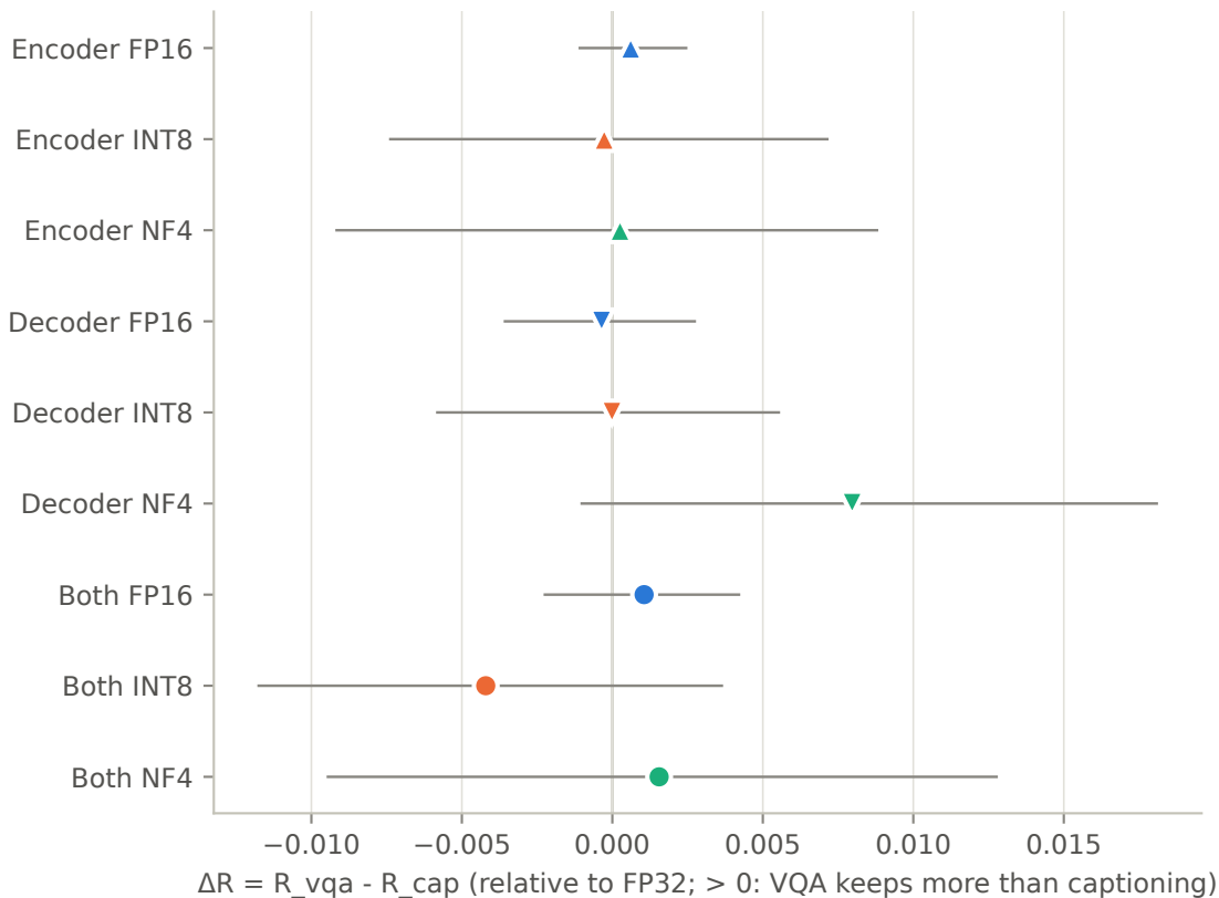
Retention under reduced precision, VQA vs captioning
