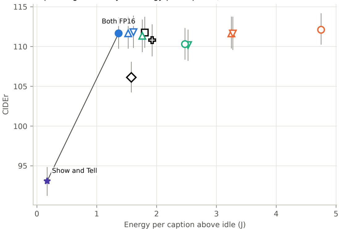
Captioning: accuracy vs energy per caption (MacBook Pro M4 Pro, batch 1)
