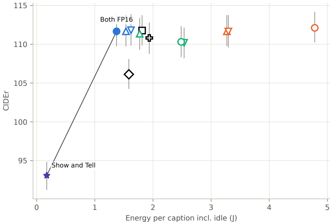
Captioning: accuracy vs energy per caption (MacBook Pro M4 Pro, batch 1, incl. idle)
