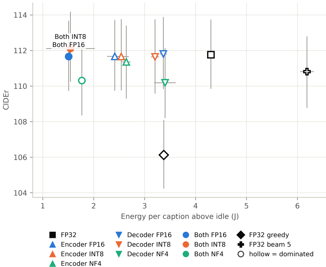
Captioning: accuracy vs energy per caption (Colab T4, batch 1)
