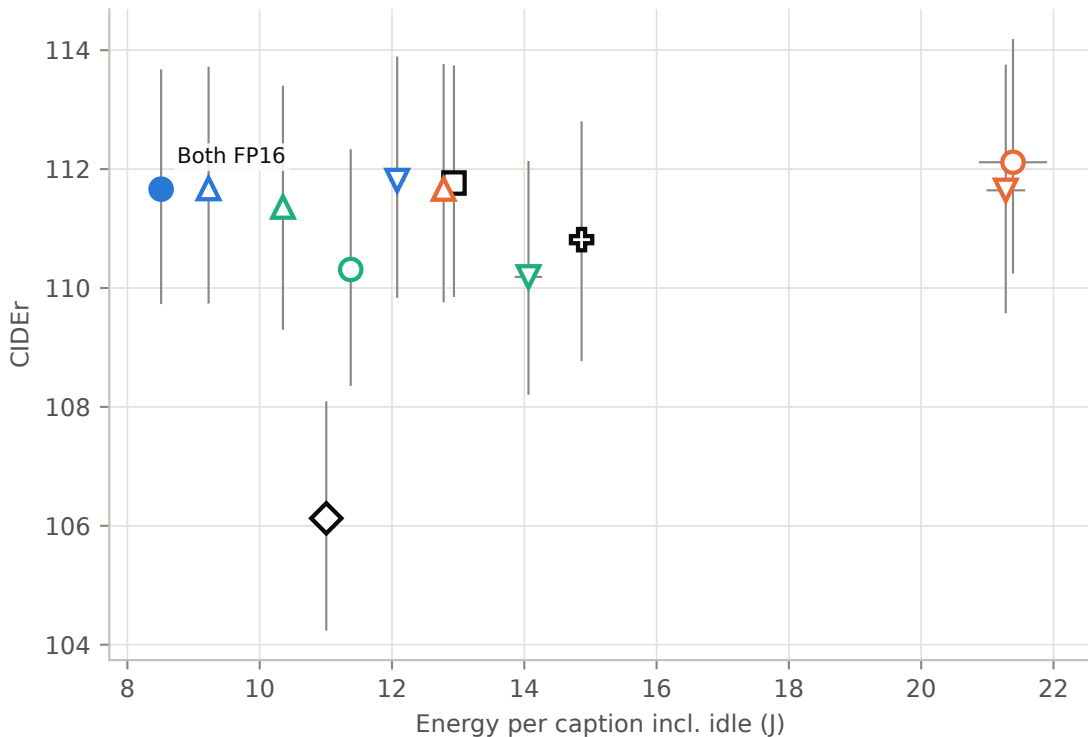
Captioning: accuracy vs energy per caption (Colab T4, batch 1, incl. idle)
