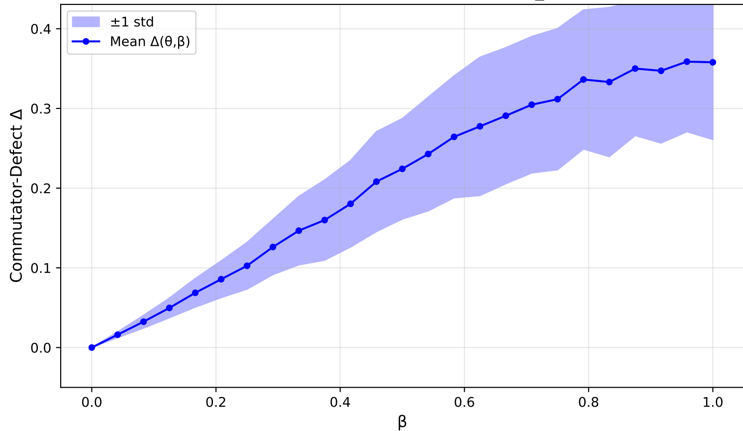
Commutator-Defect Surrogate (n=4, N_θ=300)
