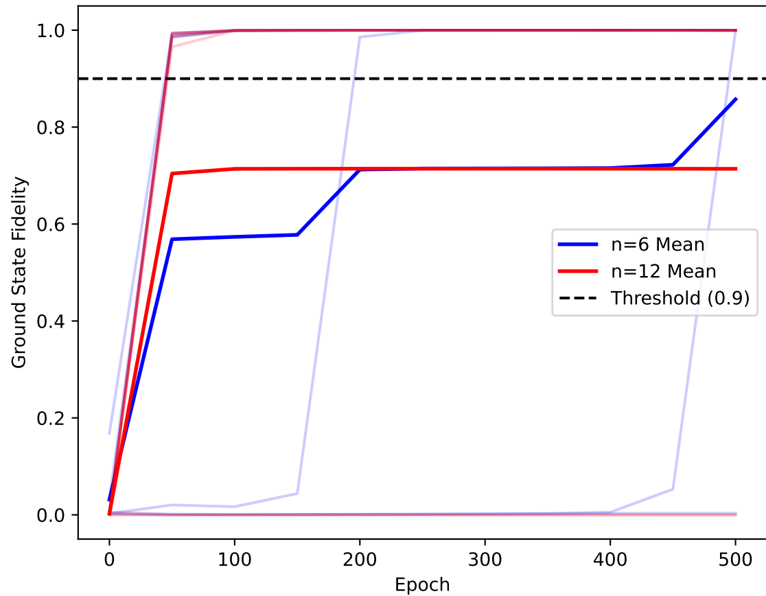
B6 (HEA, beta=1.0) Fidelity vs Epochs
