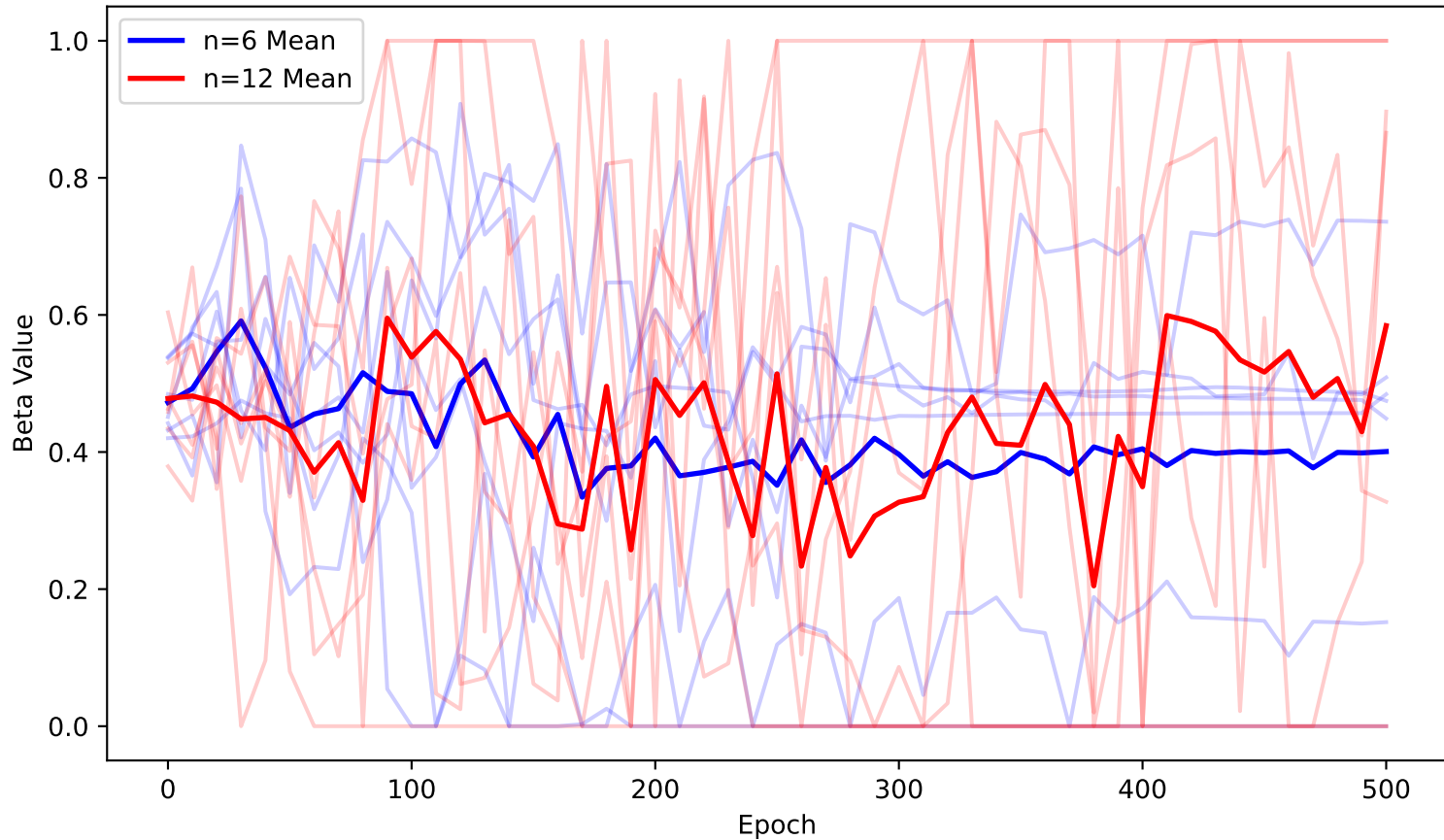
S3 Strategy: Learned Beta Trajectory
