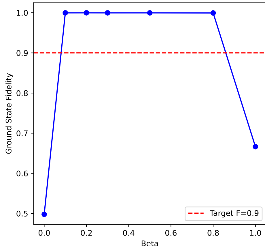
Reachability
