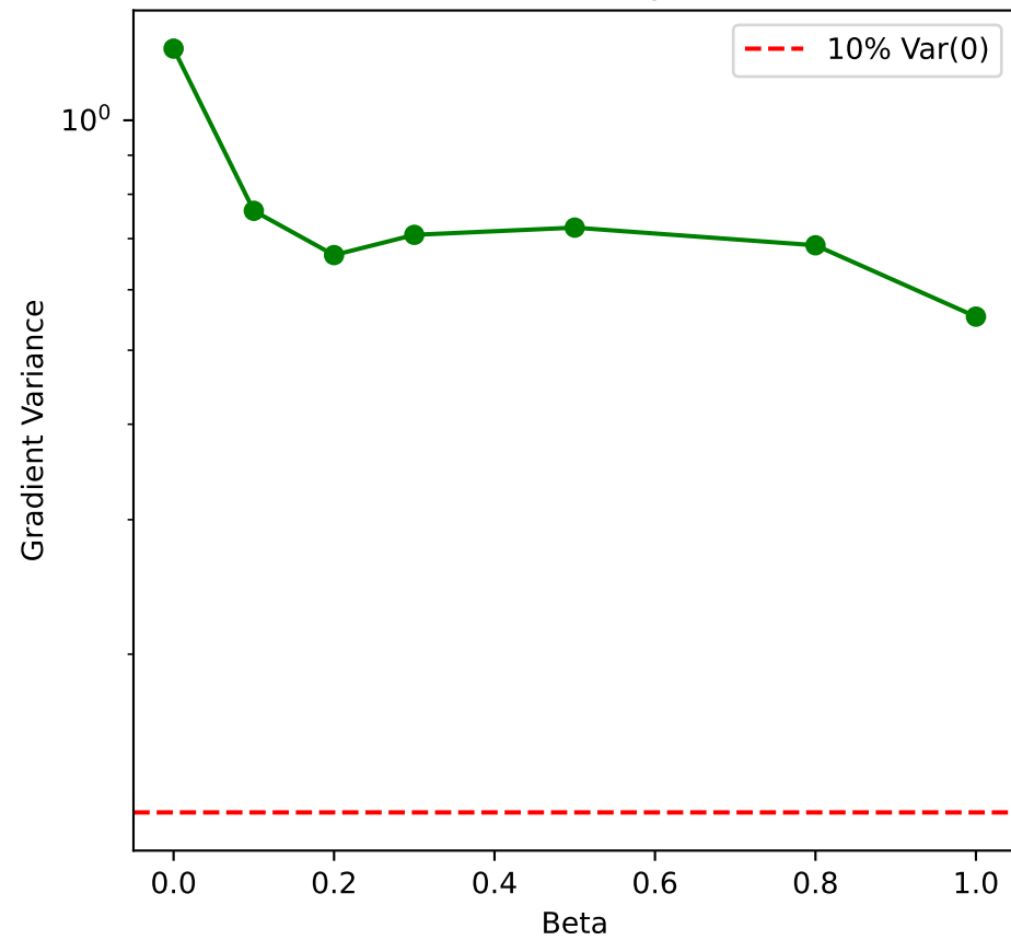
Trainability
