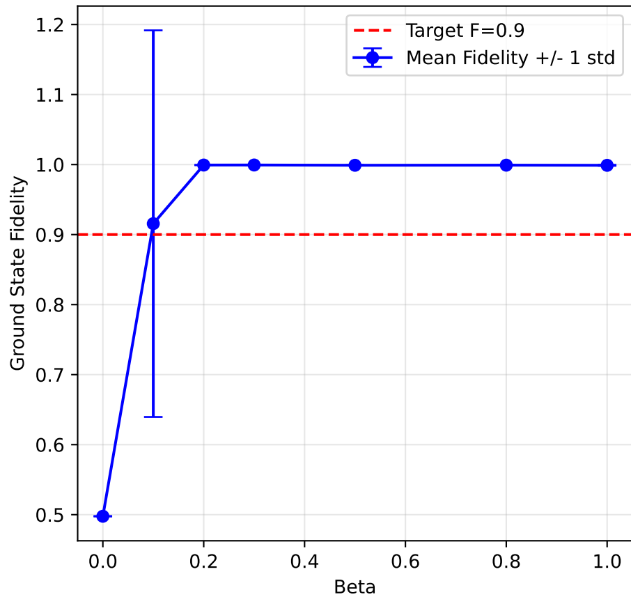
Reachability (Fidelity vs Beta)
