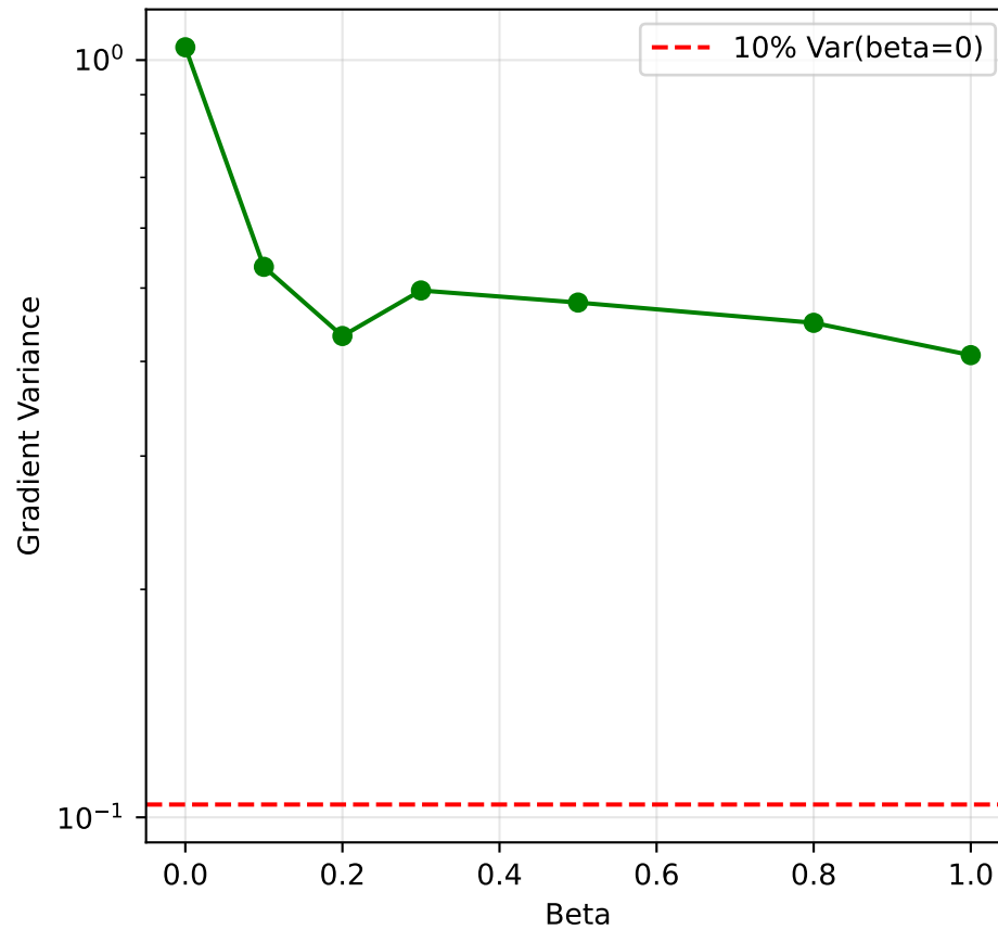
Trainability (Variance vs Beta)
